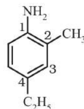
2-Chloro-4-methylanisole 4-Ethyl-2-methylaniline
