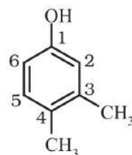
3,4-Dimethylphenol
