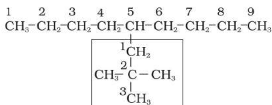
5-(2,2-Dimethylpropyl)nonane
