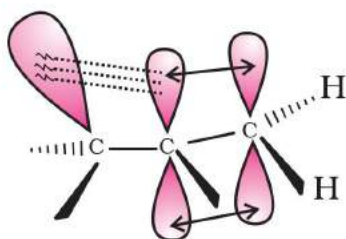
Fig. 12.4(b) Orbital diagram showing hyperconjugation in propene
