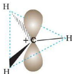
Fig. 12.3(a) Shape of methyl carbocation
