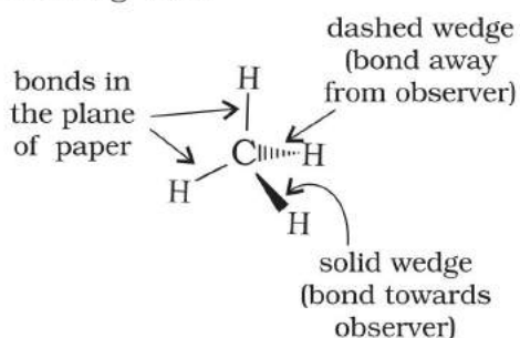
Fig. 12.1 Wedge-and-dash representation of \text{CH}_4
