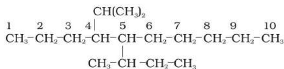
5-sec-Butyl-4-isopropyldecane
