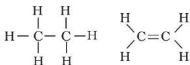
Ethane
