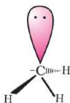
Fig. 12.3(b) Shape of methyl carbanion
