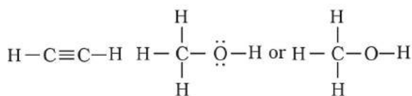
Ethyne
